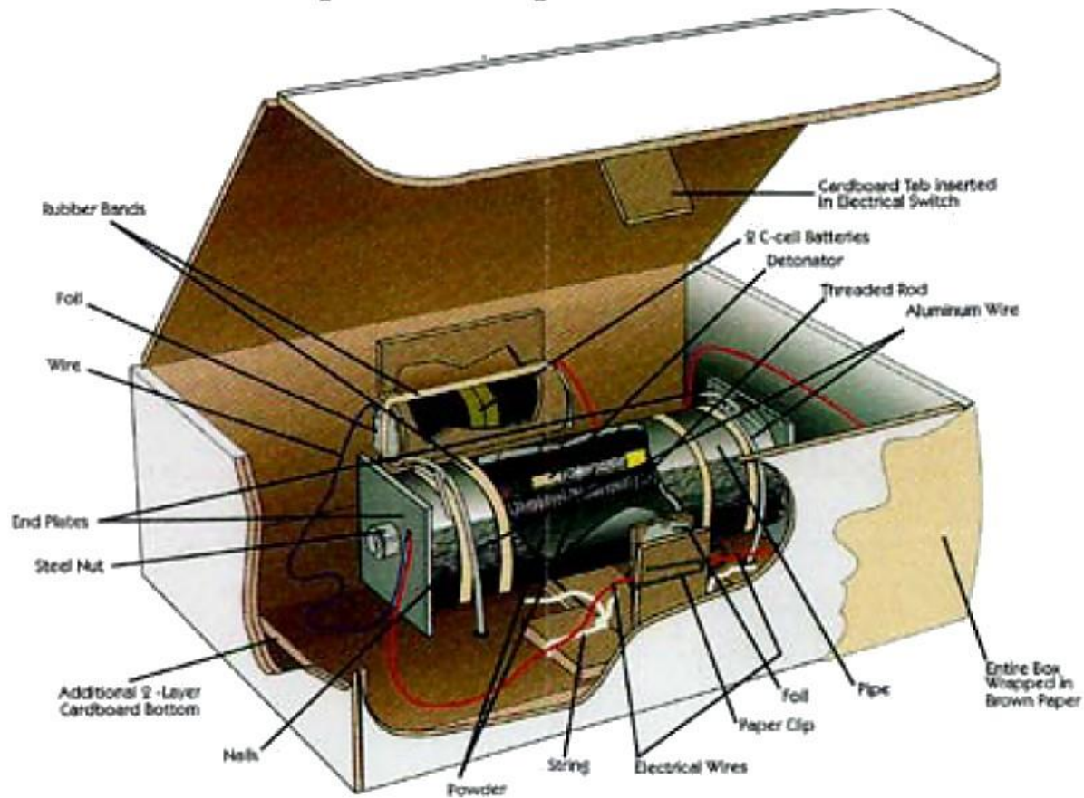
Improvised Explosive Device
